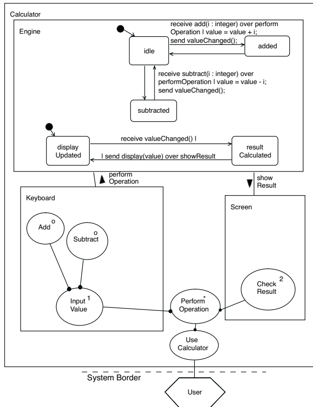
Figure 2. The corresponding simple calculator model to Fig. 1.
