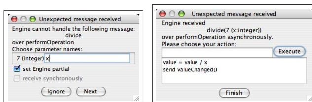
Figure 6. Reception and reaction dialog on an unhandled event.
