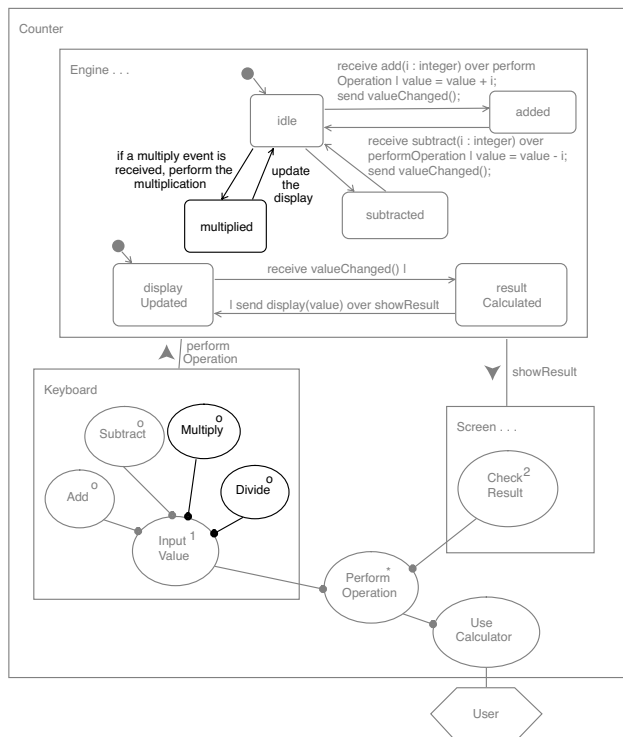
Figure 4. Incomplete and informally specified extended model. New parts are drawn in black.
