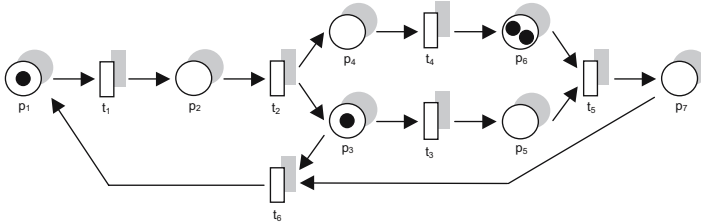
Fig. 3.3 Example of a Petri net
