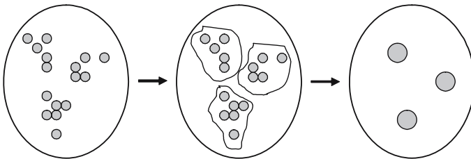
Fig. 3.8 Abstraction levels
