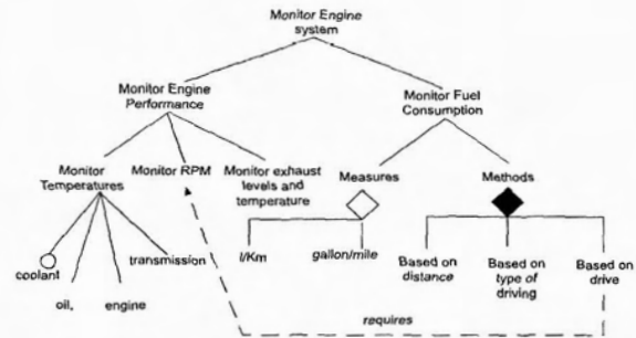
Figure 2. FeaturSEB (RFD): Monitor Engine System
