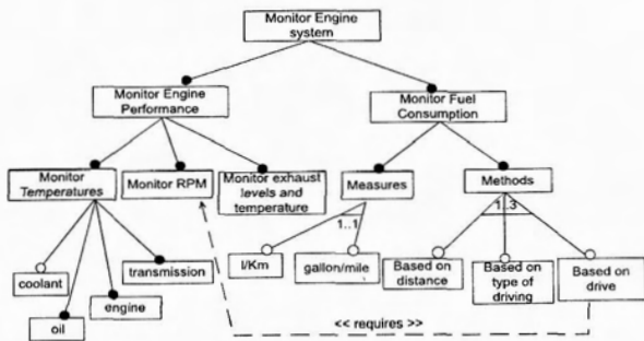
Figure 3. EFD: Monitor Engine System
