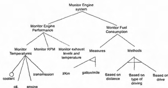
Figure 1. FODA (OFT): Monitor Engine System
