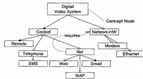
Figure 8. RFD example from [22, Fig.3]
