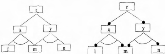
Figure 7. Node- vs. edge-based semantics
