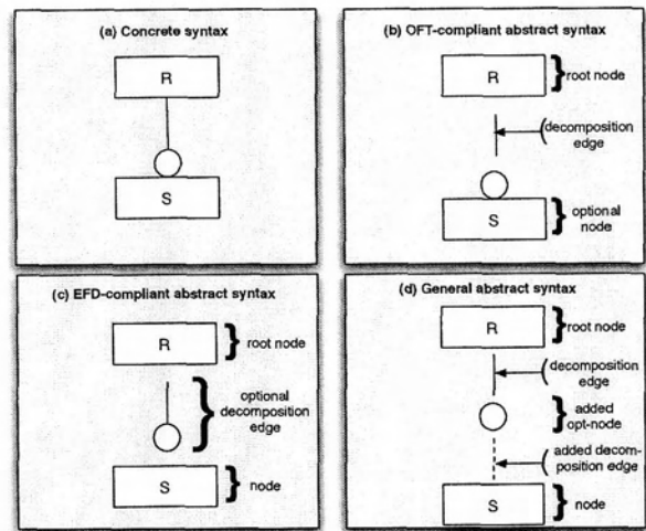
Figure 6. Three possible abstract syntaxes
