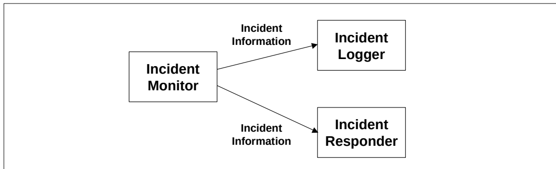
Figure 5: Requirements Objects and Information Exchanges
