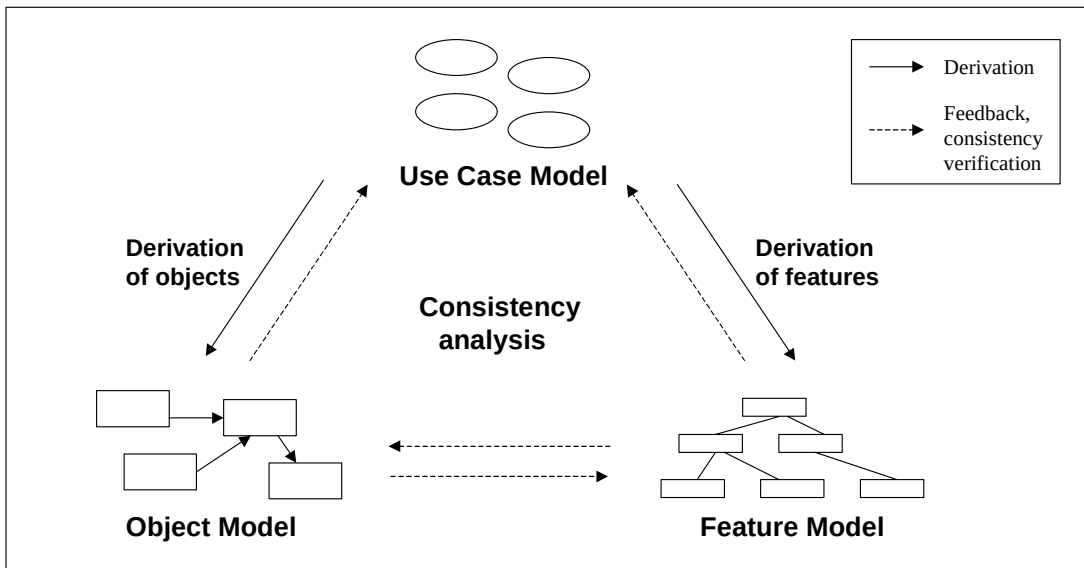
Figure 11: Model Relationships Under the Use-Case-Driven Strategy
