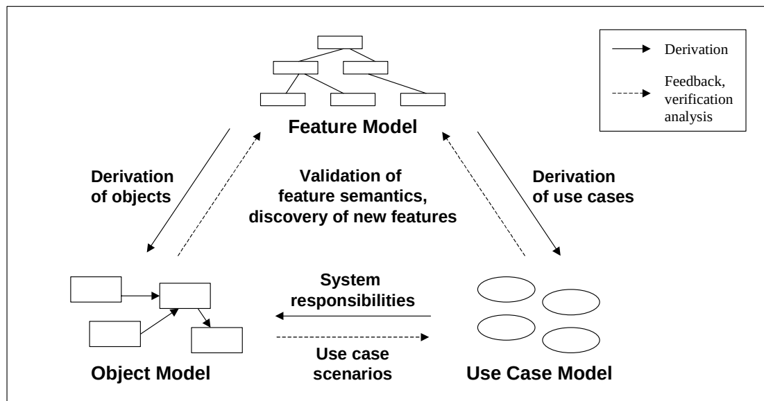
Figure 10: Model Relationships Under the Feature-Driven Strategy
