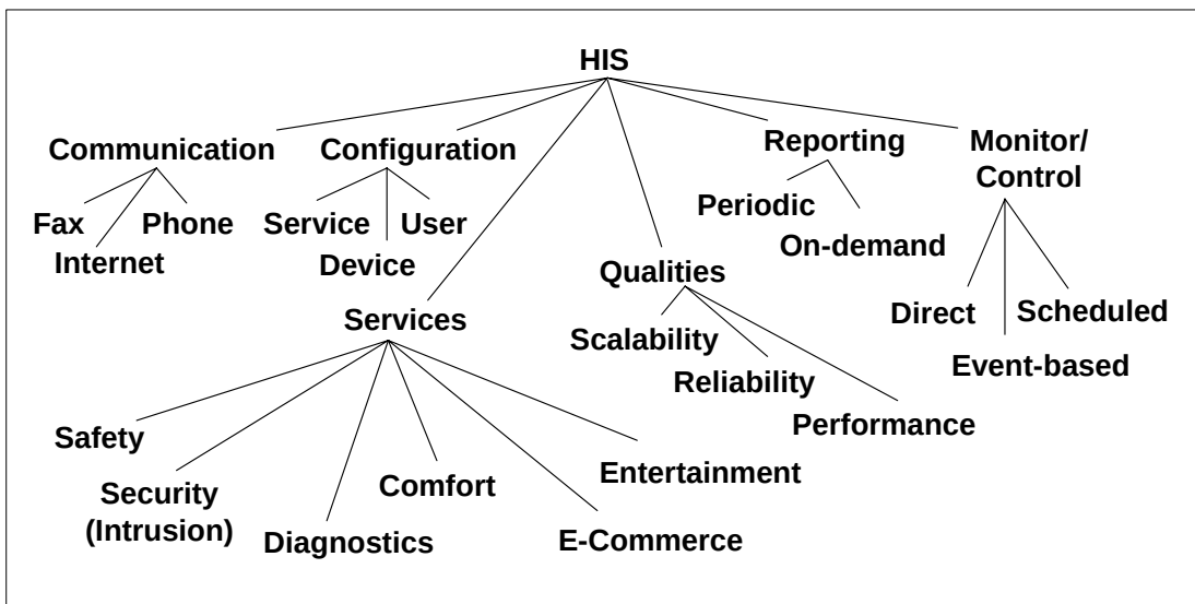
Figure 6: HIS Feature Model – Upper Levels
