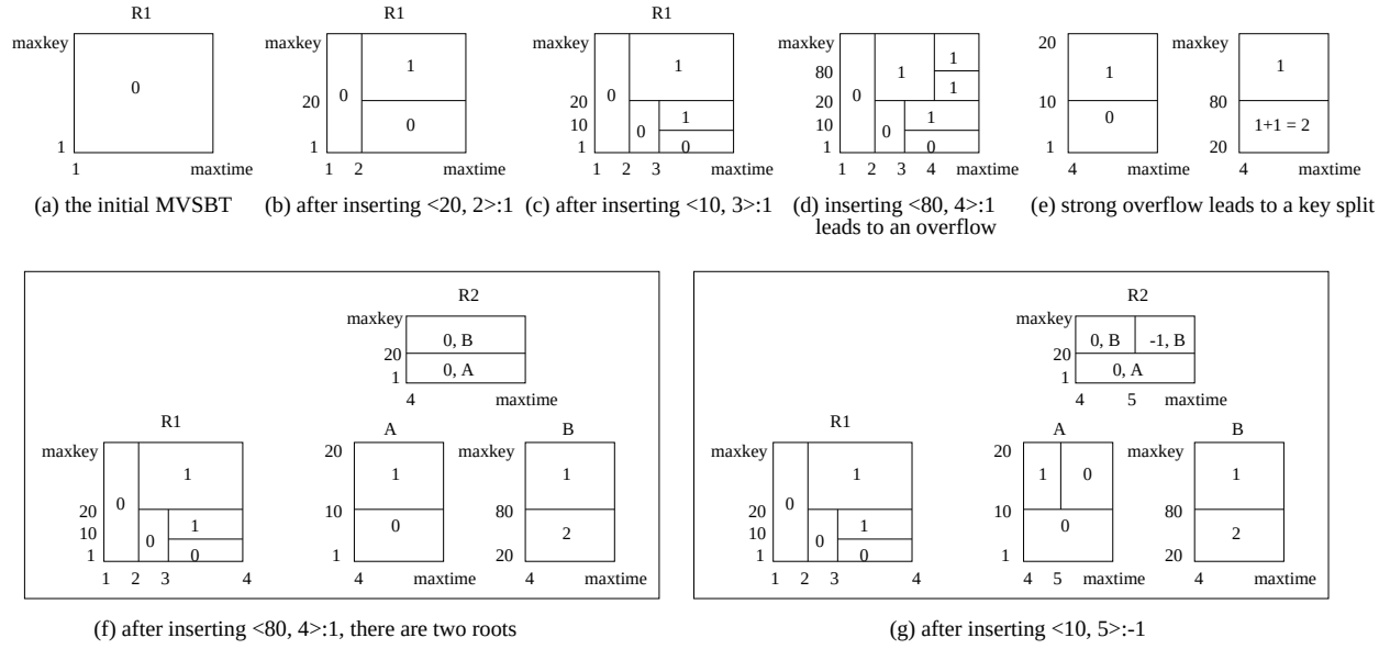
Figure 3: An example of insertions in an MVSBT
