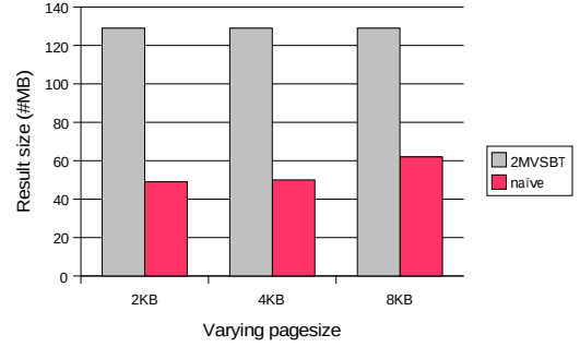
Figure 4: Comparison of Space.
