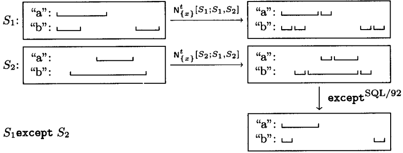
Fig. 4. Set Difference using Normalization.
