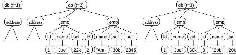
Figure 1: A sequence of versions
