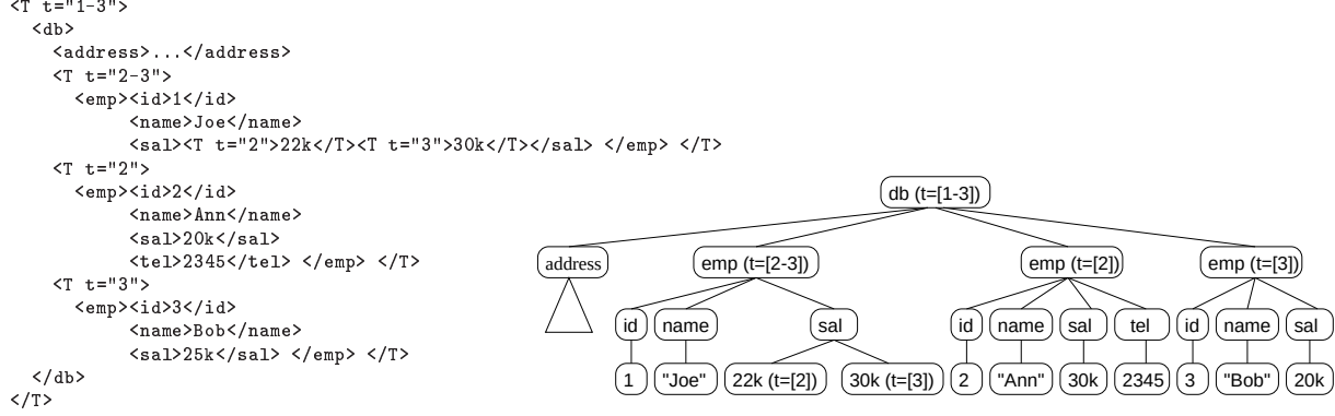
Figure 2: “Pushing” time down. Example of an archive.
