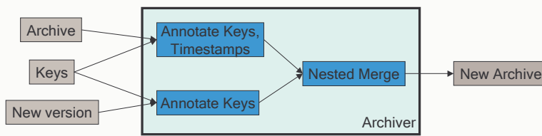
Figure 3: Main modules in our archiver
