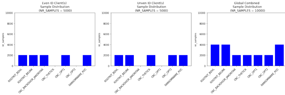
Figure 4.7: Medium Client Exclusive Sample Distribution
