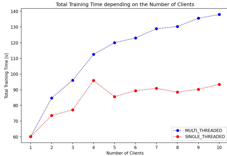
Figure 5.3: Total training time depending on the number of clients (Single vs. Multi-Threading)
