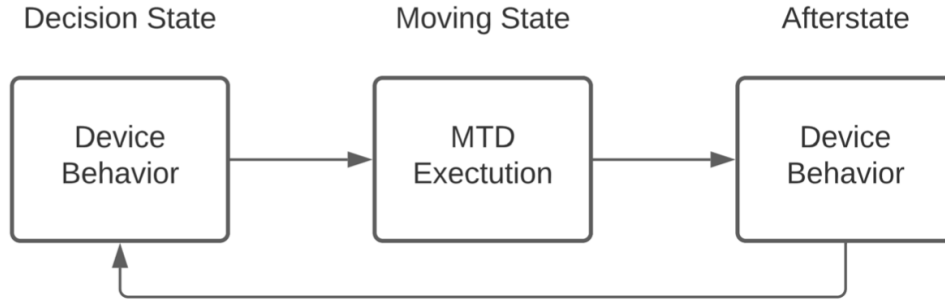
Figure 4.1: Decision and Afterstate in MTD deployment [68]
