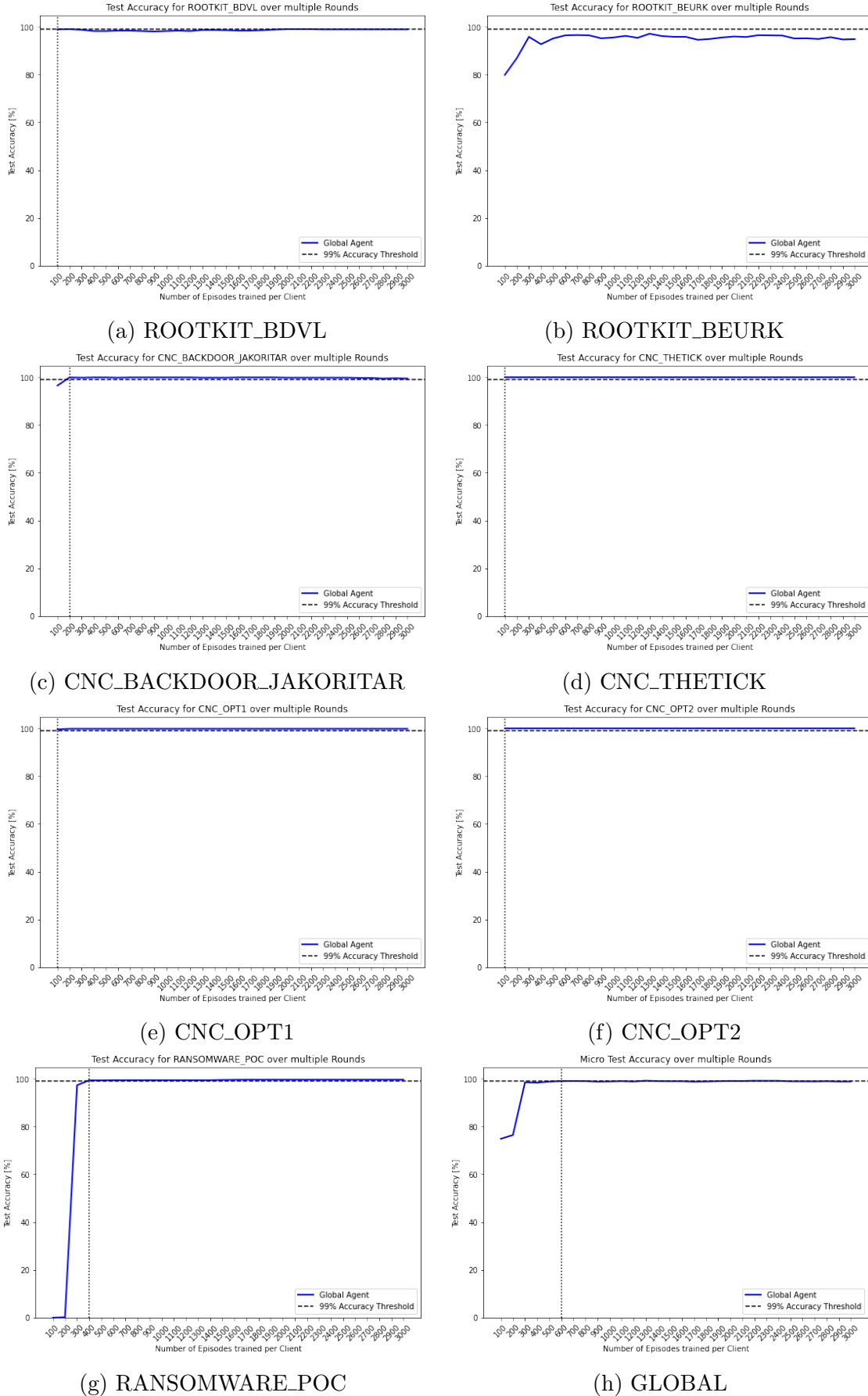
Figure 5.7: Prototype 01 Federated Training Baseline (Attack Mitigation Performance over multiple Training Rounds)
